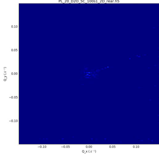
PL_20_D2O_5C_100s1_2D_rear.h5
