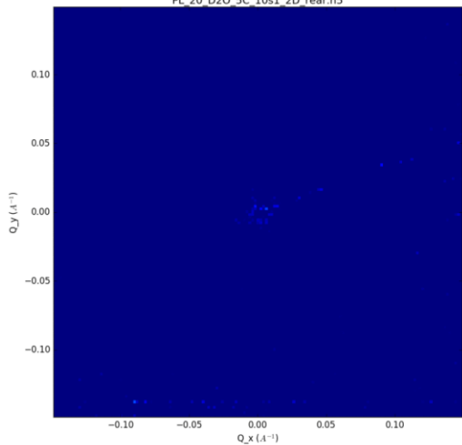
PL_20_D2O_5C_10s1_2D_rear.h5
